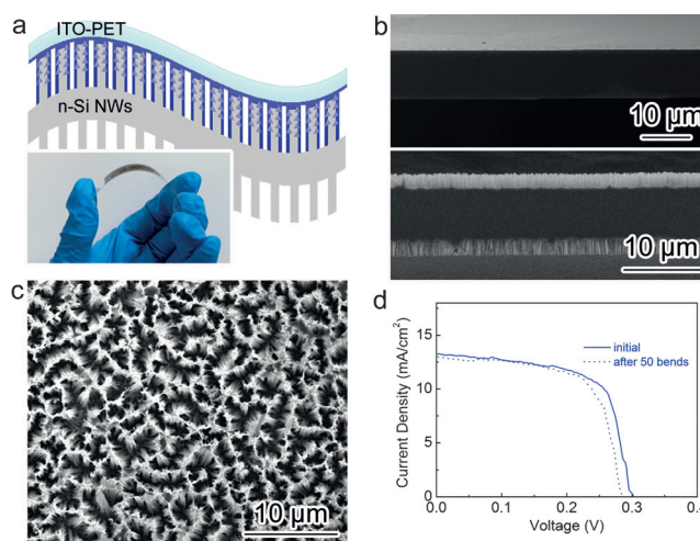
Figure 4. a) Structure of flexible n-Si NWs/Ag NPs/PEDOT:PSS device, fabricated from 10 μm thick Si film. The inset shows the photograph of a flexible device. b) Side-view SEM images of the Si ultrathin wafer (top panel) and nanowire arrays (bottom panel) used for fabrication. c) Top-view SEM image of the Si nanowire arrays. d) J – V curves of a flexible n-Si NWs/PEDOT:PSS device before and after 50 bends.
